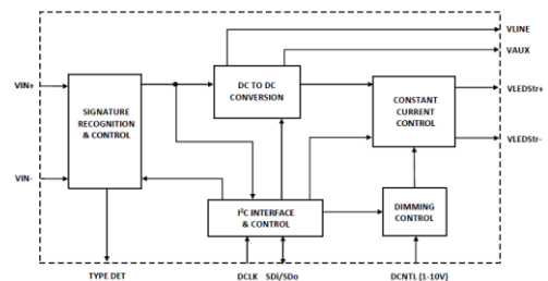
Ag210 – Block Diagram
