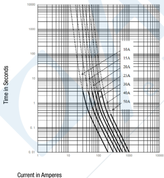
ADO PCB version, 850 VDC
