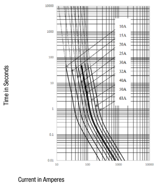
ADO PCB version, 500 VDC
