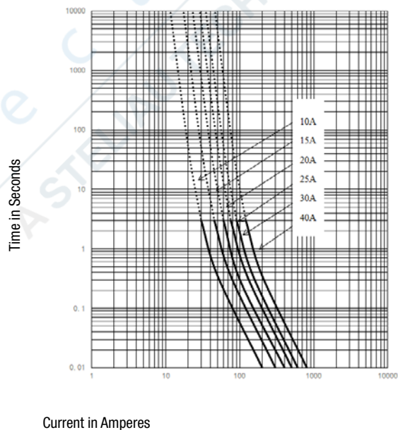
ADO PCB version, 1000 VDC
