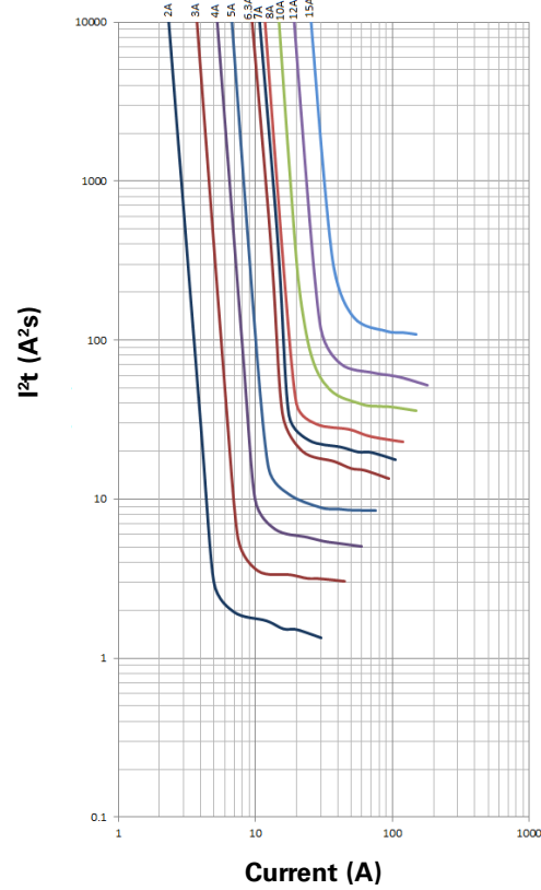
I 2 t vs current curve 2 A and 3 A and 4 A to 15 A
