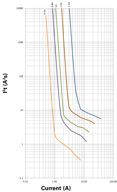
I 2 t vs. current curve 0.5 A to 1.5 A and 2.5 A
