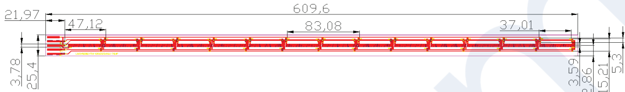
Figure 16: Drawing Overview for 610mm
