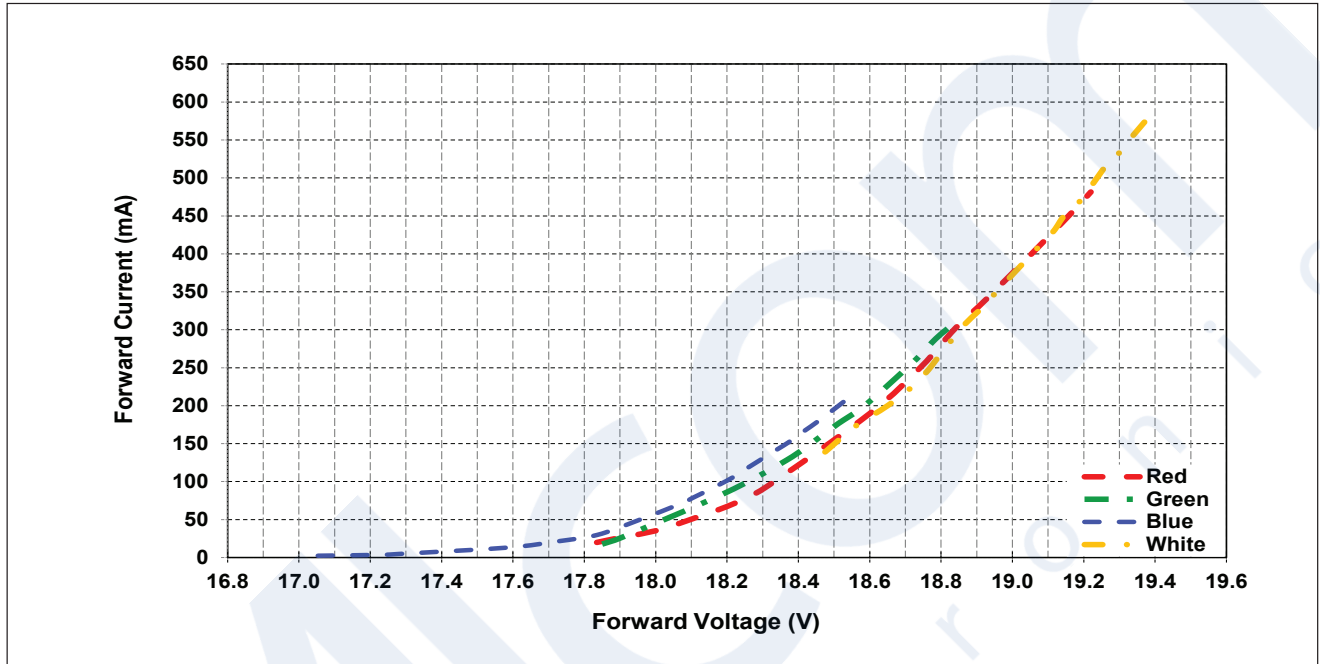
Figure 9: Drive Current Per channel vs. Voltage ( T_c = 25^\circ\text{C} ) for BXEB-L0610
