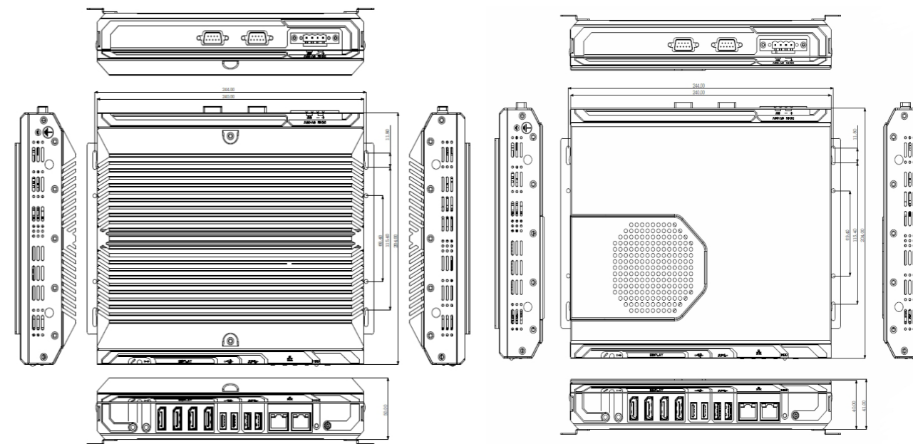
ELIT-1270-1605 (fan-less)
