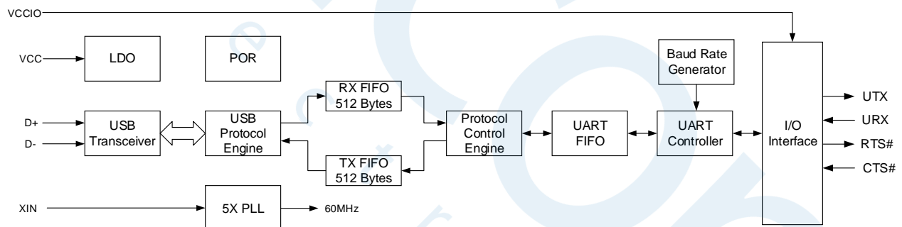
Figure 1-1 GWU2U Structure View
