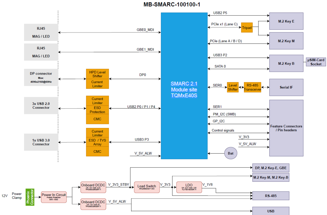
Figure 1: Block diagram MB-SMARC-100100-1
