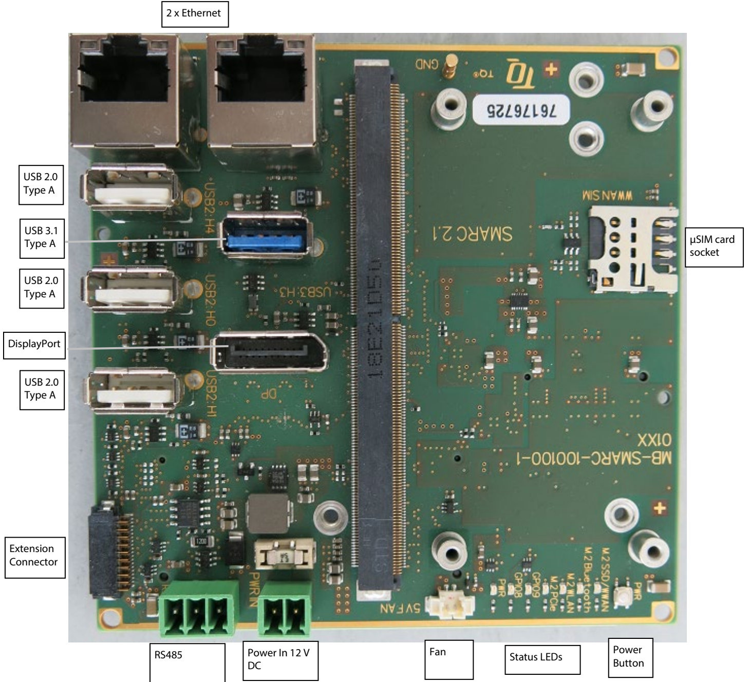
Figure 2: MB-SMARC-100100-1, Top
