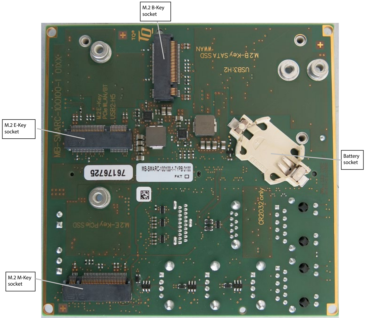
Figure 3: MB-SMARC-100100-1, Bottom
