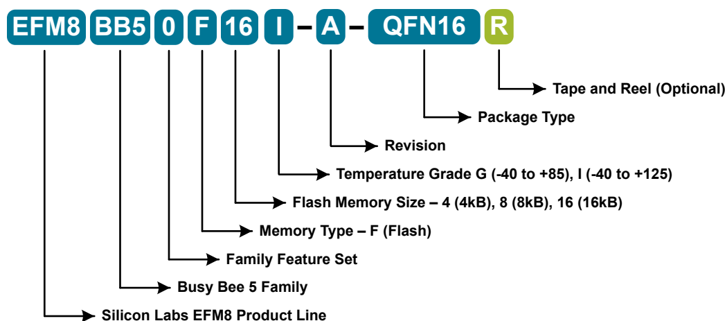
Figure 2.1. EFM8BB50 Part Numbering
