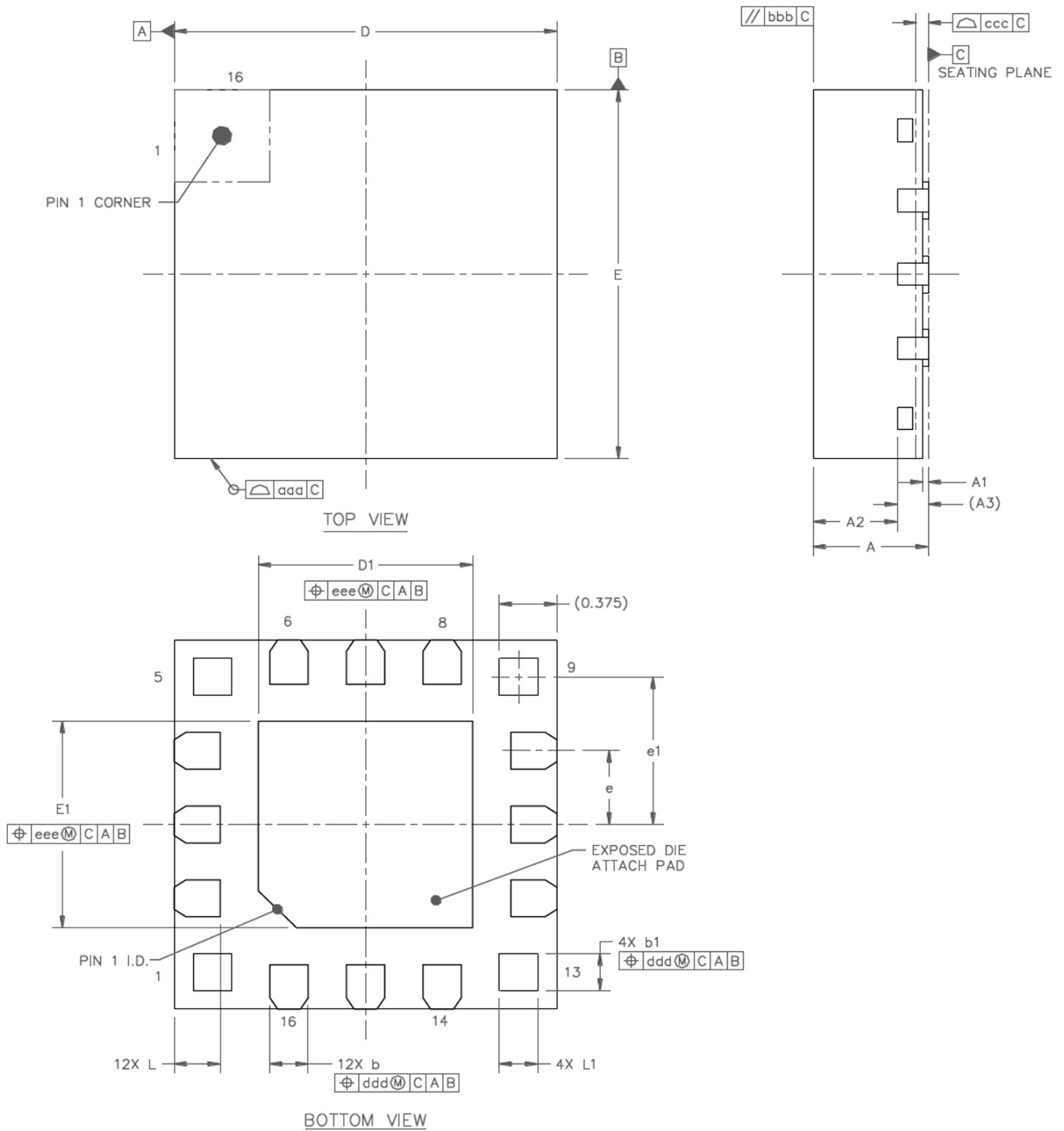
Figure 7.1. QFN16 Package Drawing
