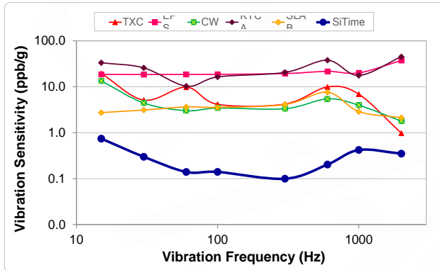
Figure 5. Vibration Robustness [5]
