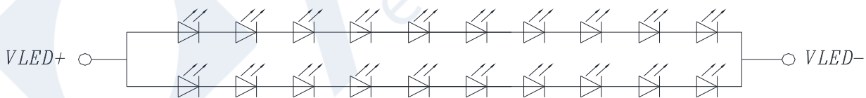
CIRCUIT DIAGRAM(LED 2*10=20 DIES)
