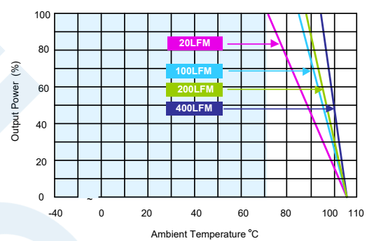
MTQZ50-72S24,MTQZ50-110S12,MTQZ50-110S24 Derating Curve with Heatsink
