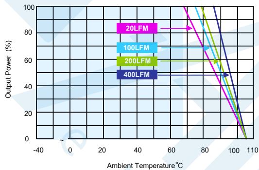
MTQZ50-72S24,MTQZ50-110S12,MTQZ50-110S24 Derating Curve without Heatsink
