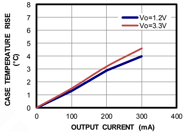
T RISE vs. Output Current
