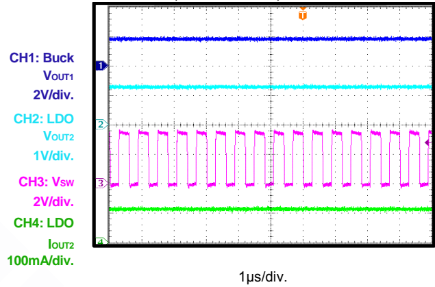
Buck+LDO
