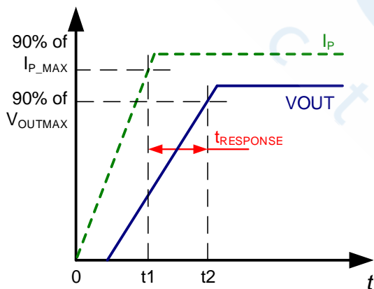
Figure 8: Response Time ( t_{RESPONSE} )
