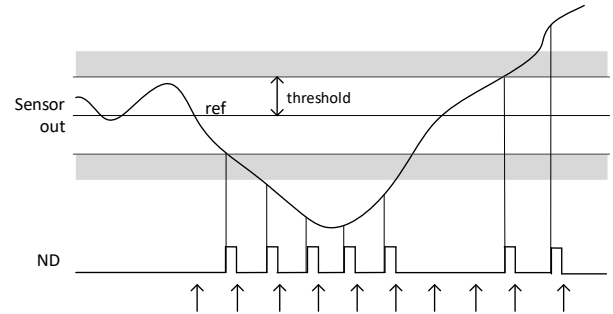
Figure 39: Example of ND signal when the Angle is Changing. Arrows indicate SPI readings.
