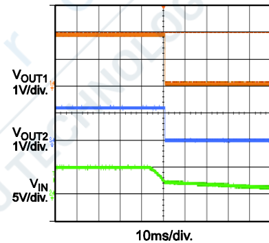
V_{IN} Power Down with 1A Load
