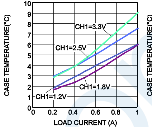
Case Temperature Rise
