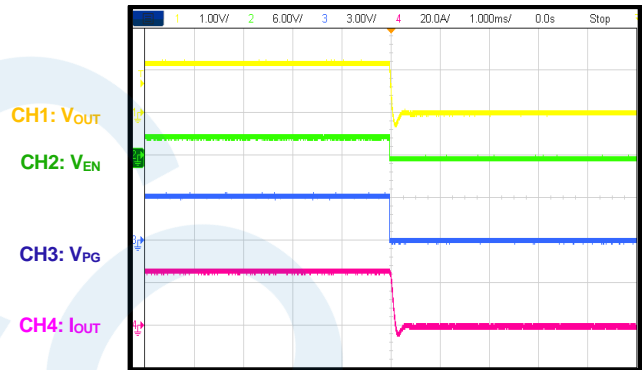
Shutdown through EN I_{OUT} = 26A
