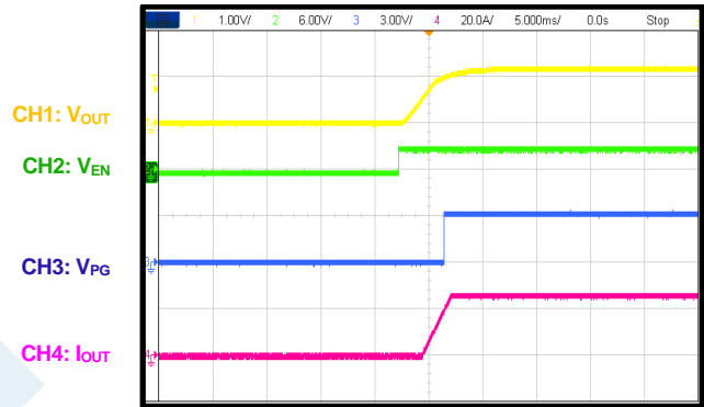
Start-Up through EN I_{OUT} = 26A
