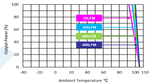
MKZI10-24S24, MKZI10-48D15 Derating Curve with Heatsink
