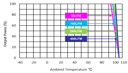
MKZI10-48D12 Derating Curve with Heatsink
