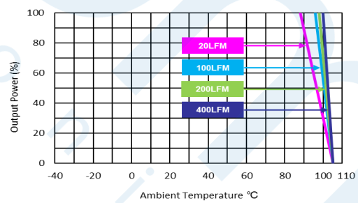
MKZI10-24S12, MKZI10-24D12, MKZI10-48S24, MKZI10-110D12 MKZI10-110D15 Derating Curve with Heatsink
