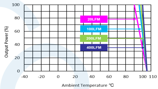
MKZI10-24S15, MKZI10-24D15, MKZI10-48S12, MKZI10-48S15 Derating Curve with Heatsink
