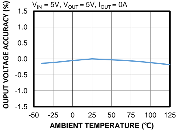
Output Voltage Accuracy vs. Temperature
