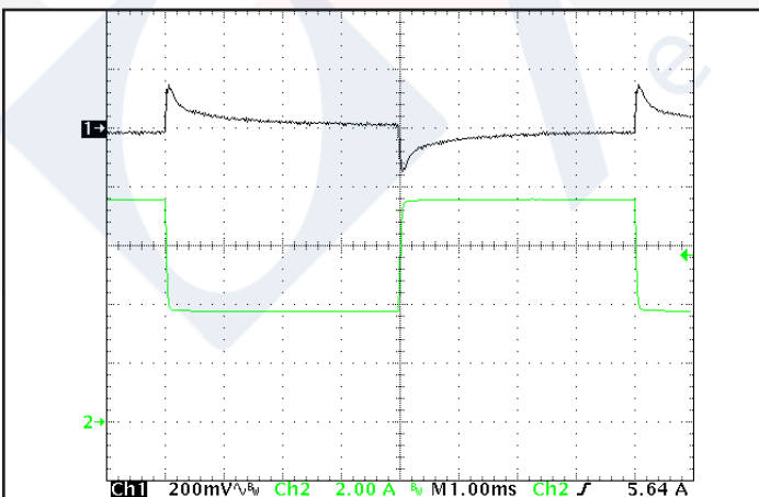
Figure 11: Output voltage response to step-change in load current 50%-100%-50% of Iout (max); dI/dt = 0.07 \text{ A}/\mu\text{s} . No external load capacitance. Ch 1: Vout (200 mV/div). Ch 2: Iout (2 A/div). (1 ms/div).
