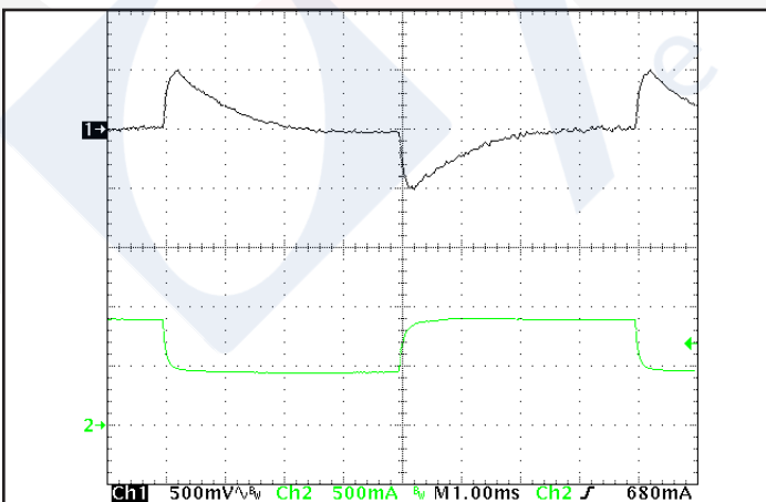
Figure 11: Output voltage response to step-change in load current 50%-100%-50% of Iout (max); dI/dt = 2 \text{ mA}/\mu\text{s} . No external load capacitance. Ch 1: Vout (500 mV/div). Ch 2: Iout (500 mA/div). (1 ms/div).
