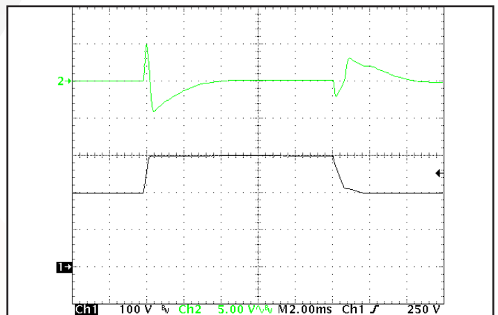
Figure 12: Output voltage response to step-change in input voltage (200 V - 300 V - 200 V); dV/dt = 400 \text{ V}/\text{ms} (rising). Ch 1: Vin (100 V/div). Ch 2: Vout (5 V/div). (2 ms/div).
