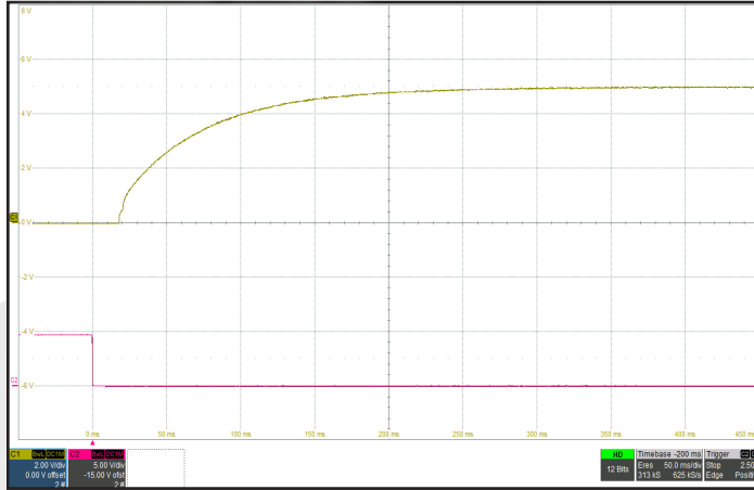
Figure 7: Turn-on transient at no load and zero output capacitance initiated by On/Off. Input voltage pre-applied. Ch 1: Vout (2 V/div). Ch 2: On/Off (5 V/div). Timescale: 50.0ms/div.
