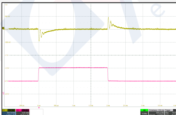
Figure 11: Output voltage response to step-change in load current 50%-100%-50% of Iout (max). No external load capacitance. Ch 1: Vout (500 mV/div). Ch 2: Iout (5 A/div). Timescale: 500μs/div.
