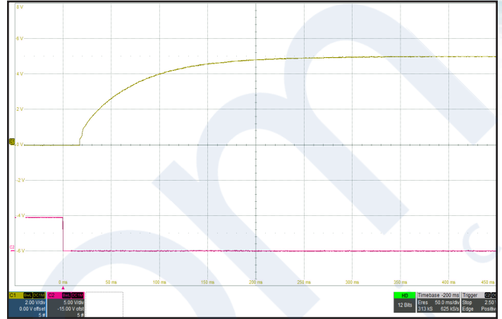
Figure 8: Turn-on transient at full resistive load and zero output capacitance initiated by On/Off. Input voltage pre-applied. Ch 1: Vout (2 V/div). Ch 2: On/Off (5 V/div). Timescale: 50.0ms/div.
