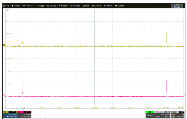
Figure 18: A short circuit across the output terminals. Ch 1: V_{out} (500 mV/div). Ch 2: I_{out} (10 A/div).
