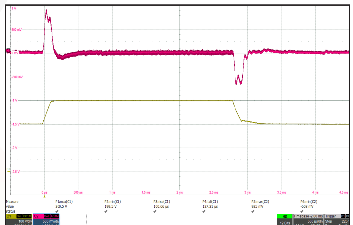
Figure 12: Output voltage response to step-change in input voltage (200 V - 300 V - 200 V) in 100 μs. Ch 2: Vout (500 mV/div). Ch 1: Vin (100 V/div). Timescale: 500μs/div.
