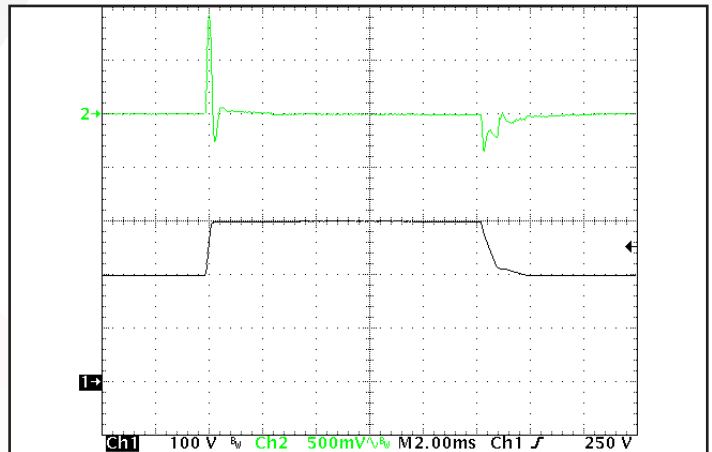
Figure 12: Output voltage response to step-change in input voltage (200 V - 300 V - 200 V); dV/dt = 500 \text{ V}/\text{ms} (rising). Ch 1: Vin (100 V/div). Ch 2: Vout (500 mV/div). (2 ms/div).
