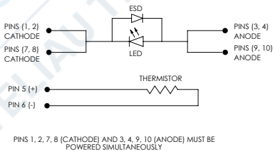
LED CIRCUIT DIAGRAM
