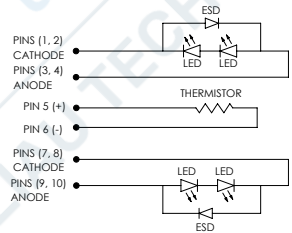
LED CIRCUIT DIAGRAM
