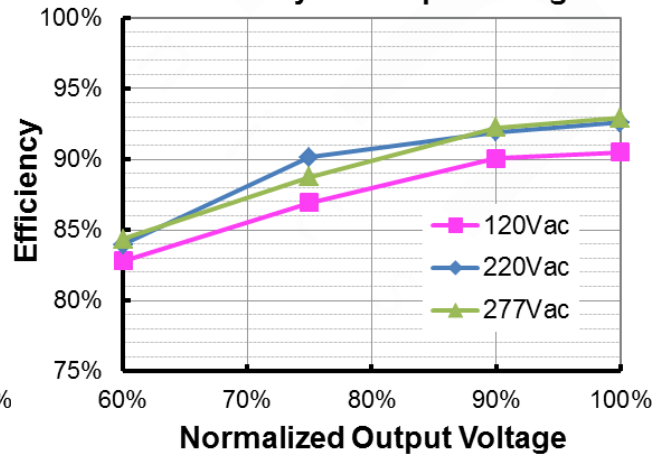
EUM-100S105Bx(I o =1050mA) Efficiency vs. Output Voltage
