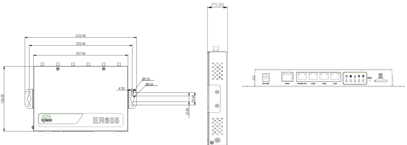
Dimensions: 198 * 137 * 25 (mm)
