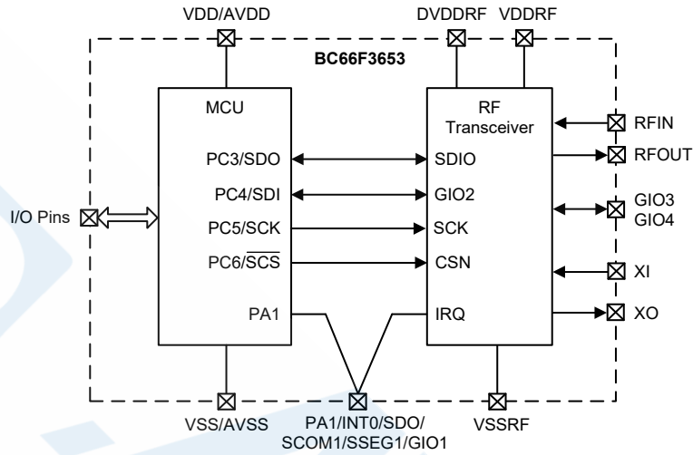
Device Connection Diagram
