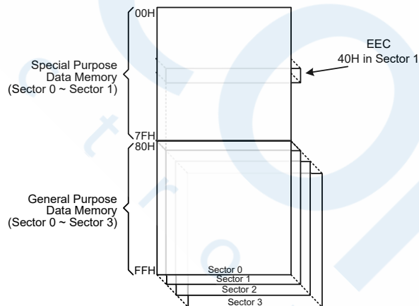
Data Memory Summary
