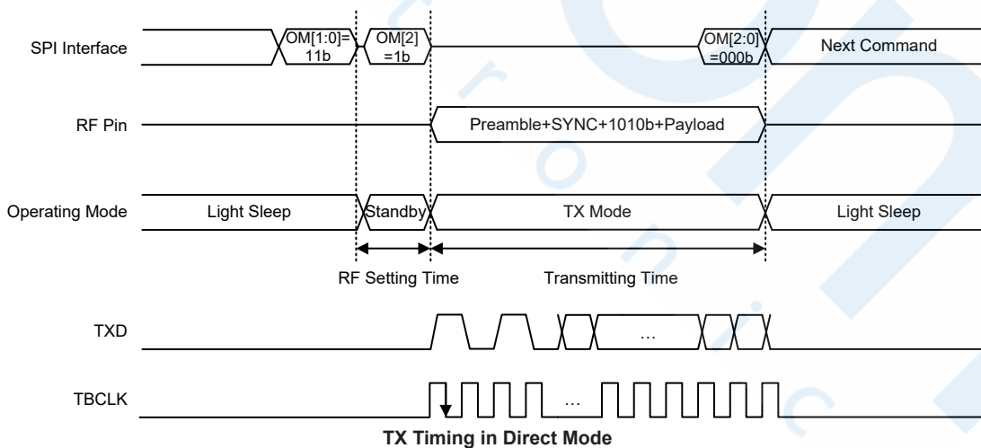
TX Timing in Direct Mode
