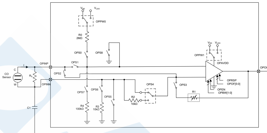
CO/Gas Detector Application Schematic
