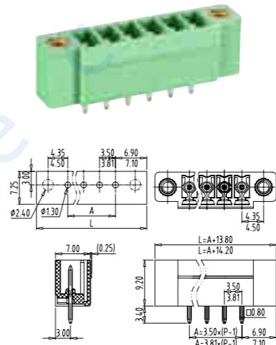
TLPHW-001V(TLPHW-100V)
