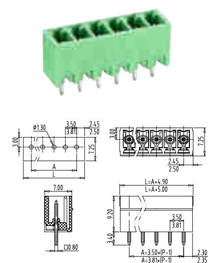
TLPHC-001V(TLPHC-100V)
