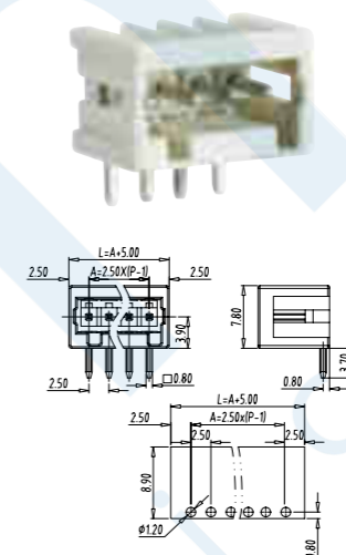
TLCH-002R
