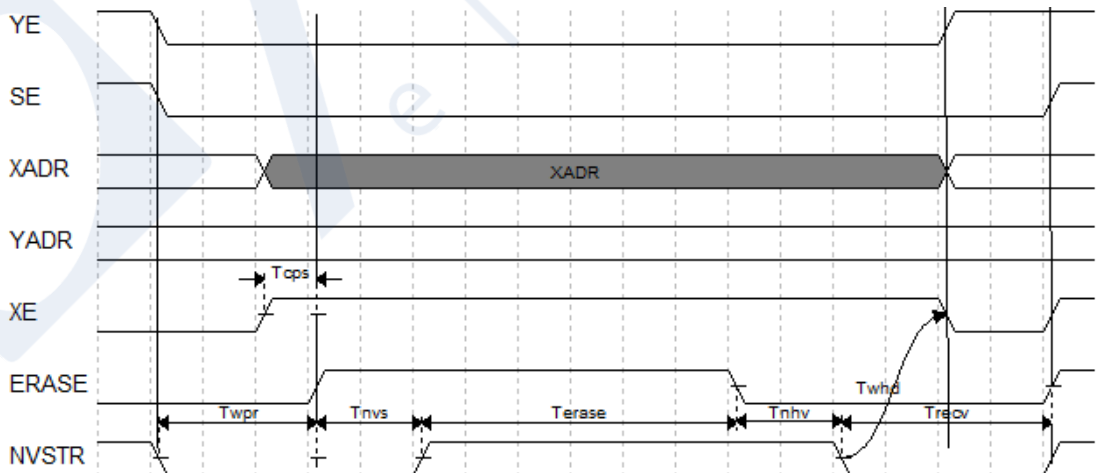
Figure 3-7 Erase Timing
