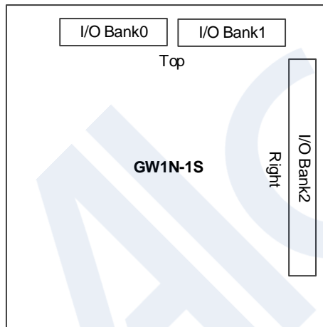
Figure 2-8 I/O Bank Distribution View of GW1N-1S
