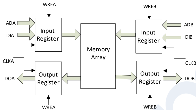
Figure 2-18 Independent Clock Mode
