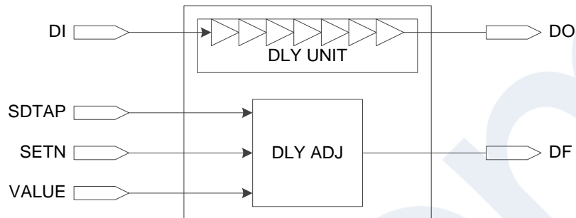
Figure 2-14 IODELAY Diagram
