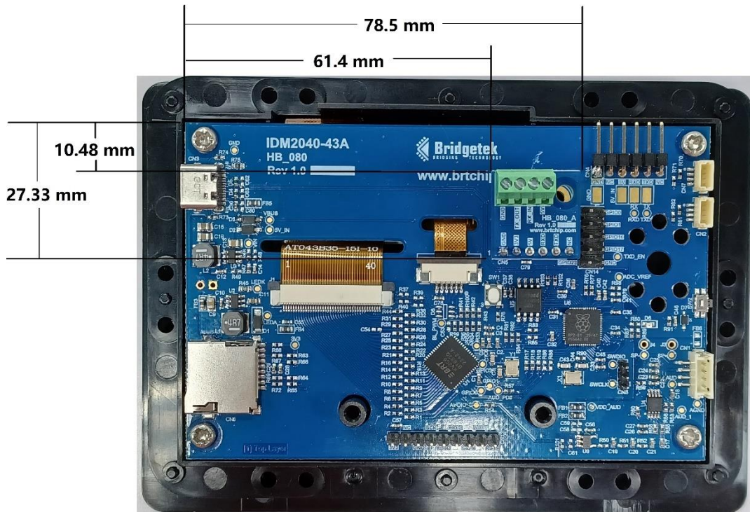
Figure 19 - IDM2040 Product Dimensions (Back View)
