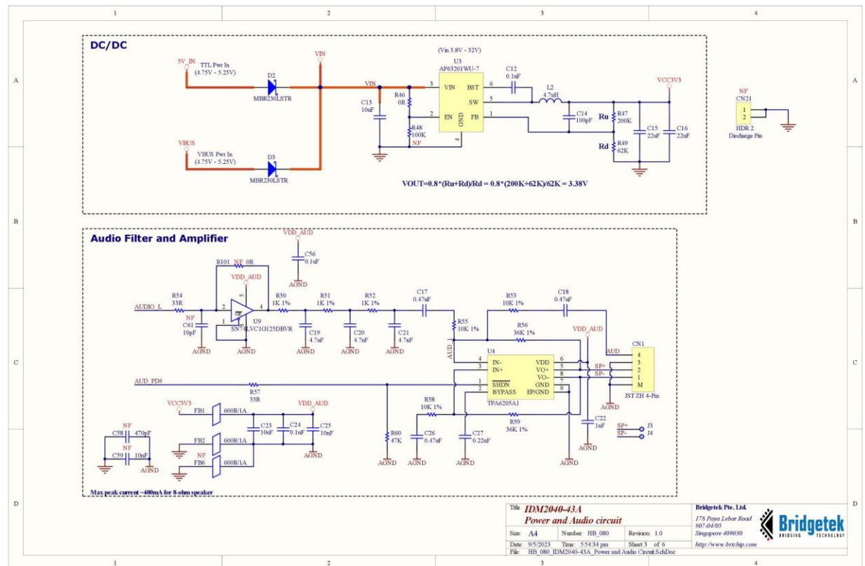
Figure 13 – Power and Audio Circuit
