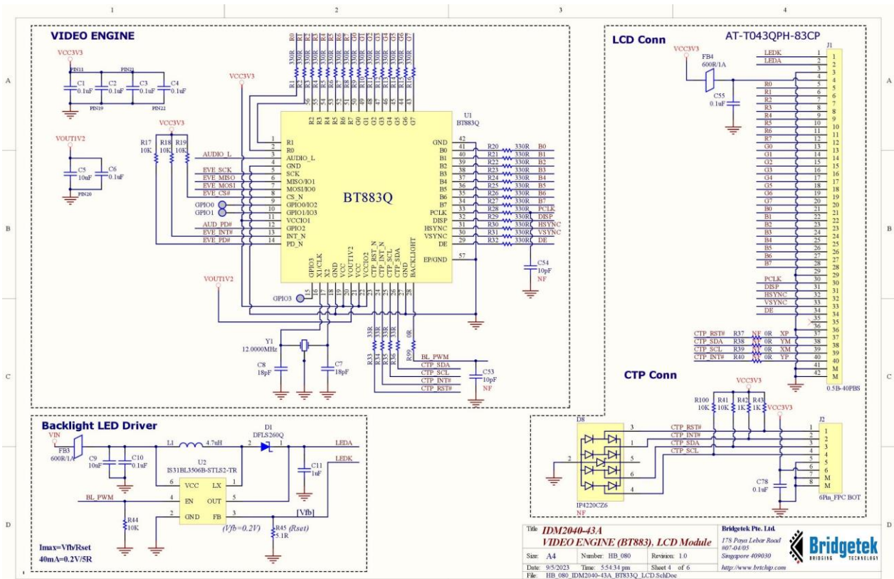
Figure 12 – BT883Q and LCD Circuit
