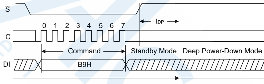
Figure 25. Deep Power-Down Sequence Diagram
