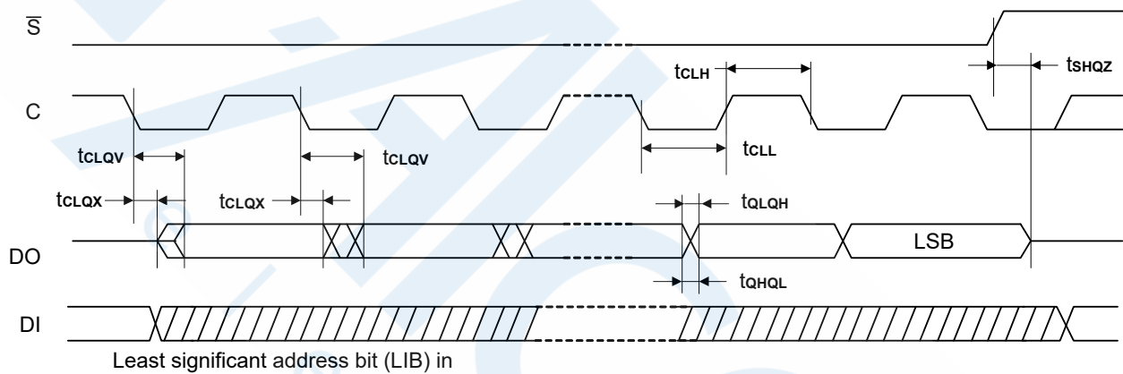
Figure 44. Output Timing
