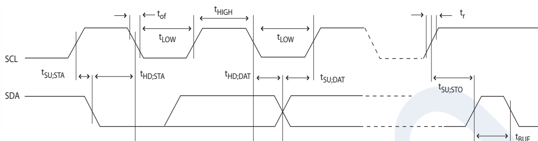
Figure 3-1. I 2 C Timings chronograms
