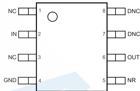
TPR70 Series SOP8 Package Top View
