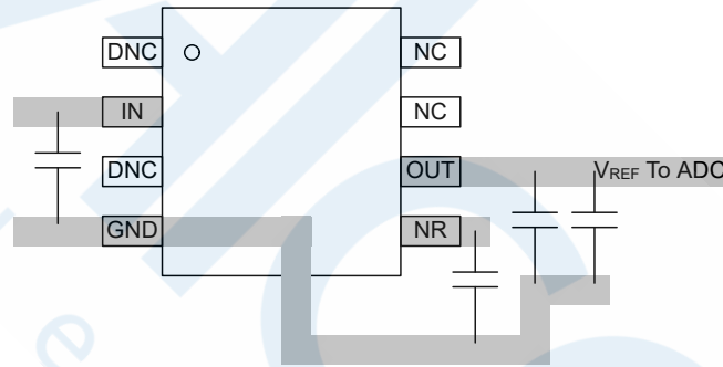
Figure 15. Layout Example
