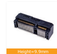
Height=9.9mm 119A-99A00-R02 Accessories 119A-NUT-99-R02, Nut 119A-SCREW-R02, Screw
